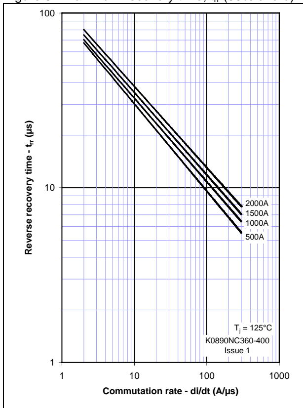
Figure 8 - Maximum recovery time, t_r (50% chord)
